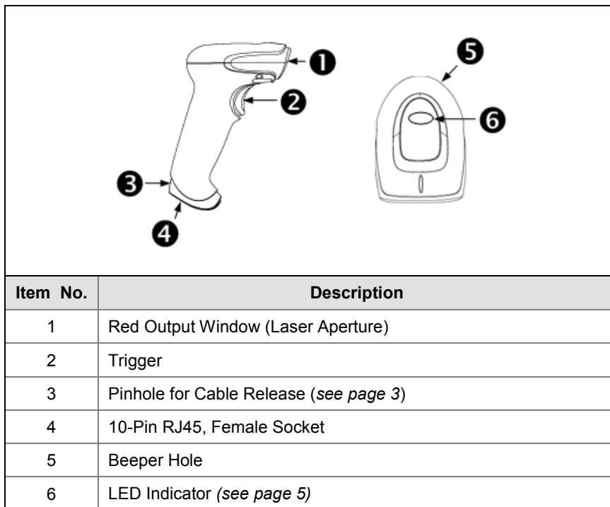
Figure 1. Scanner Components
